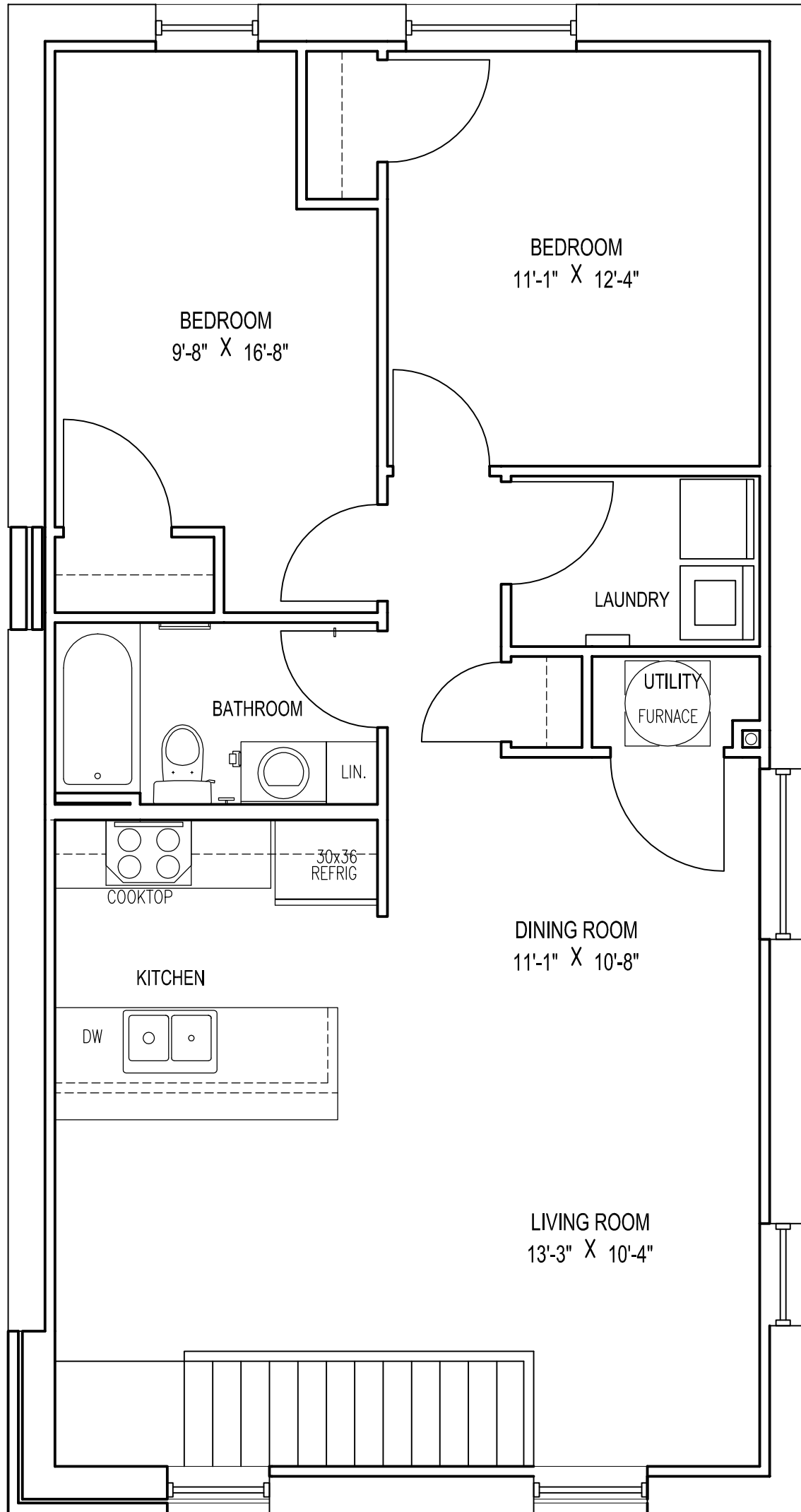
4100 ST. FERDINAND GARDEN UNIT - 2ND FLOOR
