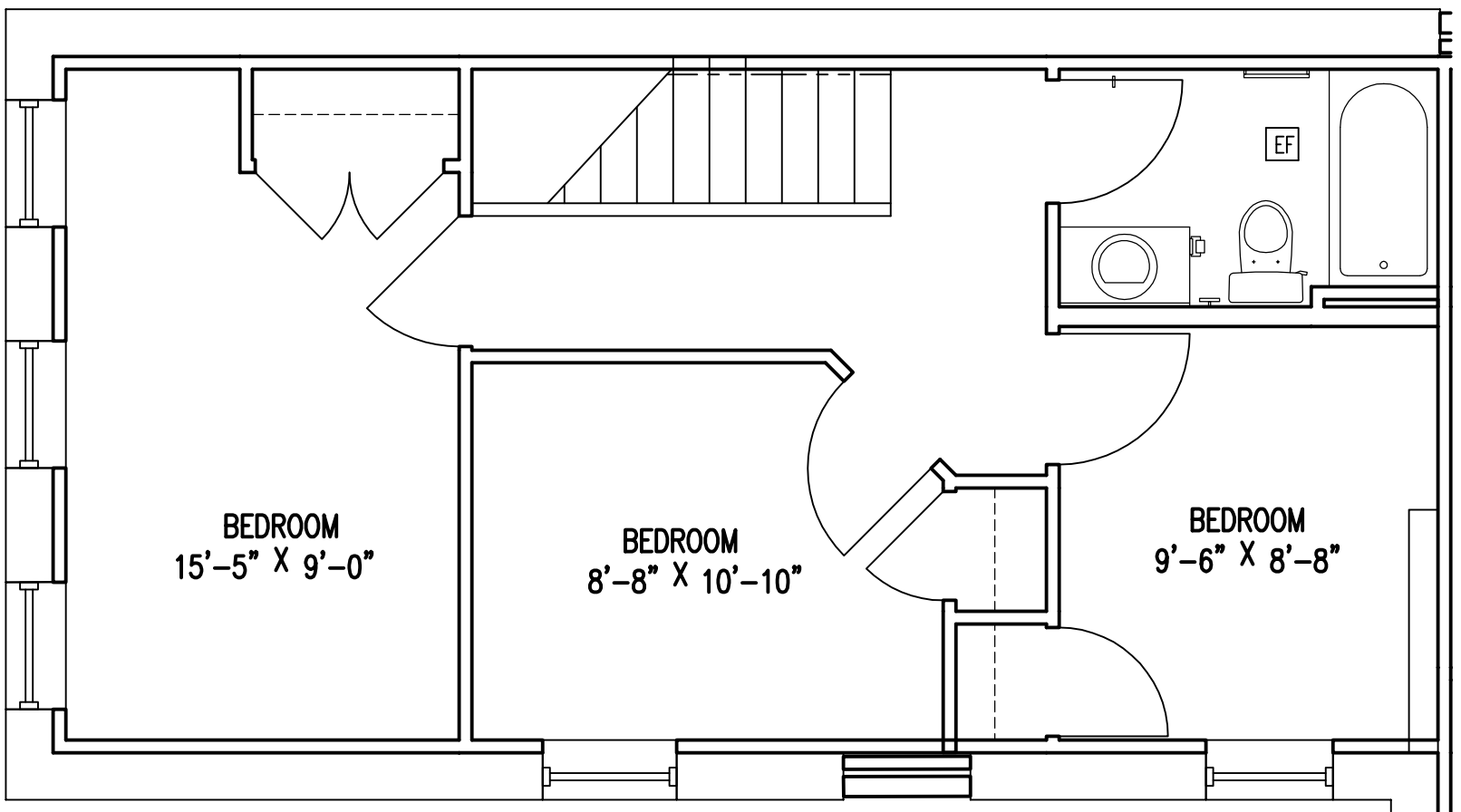
2510 N. SARAH TOWNHOME - 2ND FLOOR
