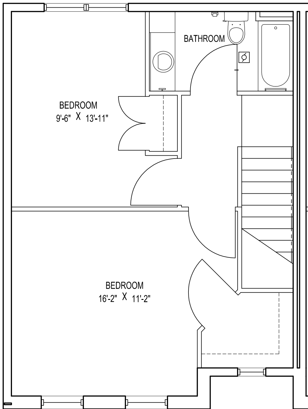
NEW CONSTRUCTION TOWNHOME 3 - 2ND FLOOR
