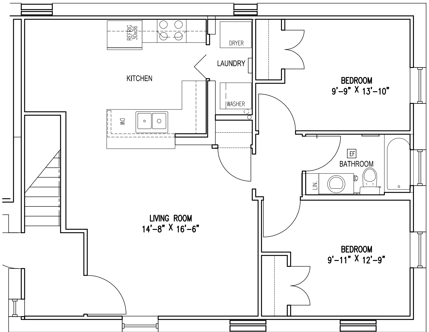
2510 N. SARAH GARDEN UNIT - 1ST FLOOR
