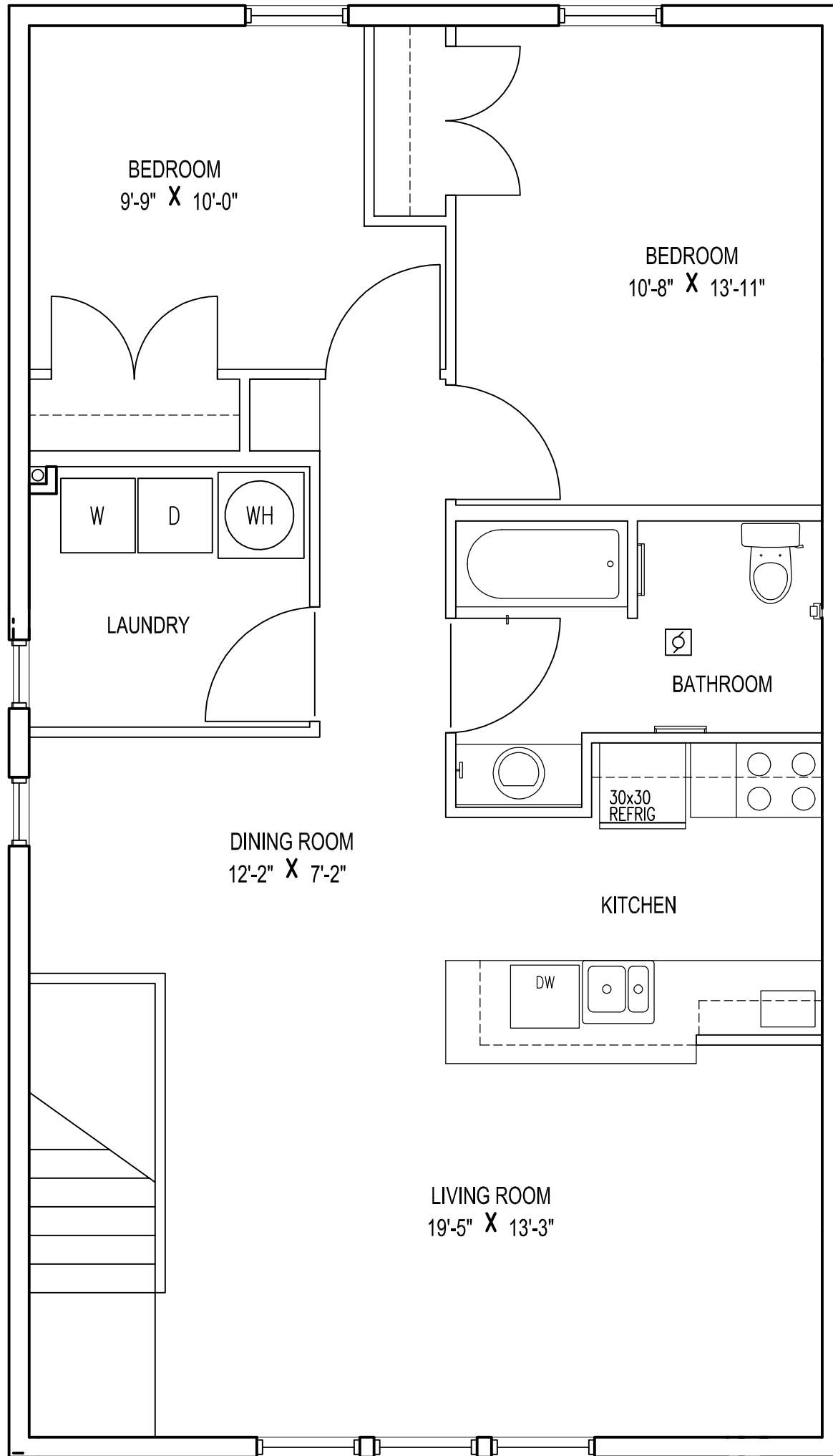
NEW CONSTRUCTION GARDEN UNIT - 2ND FLOOR
