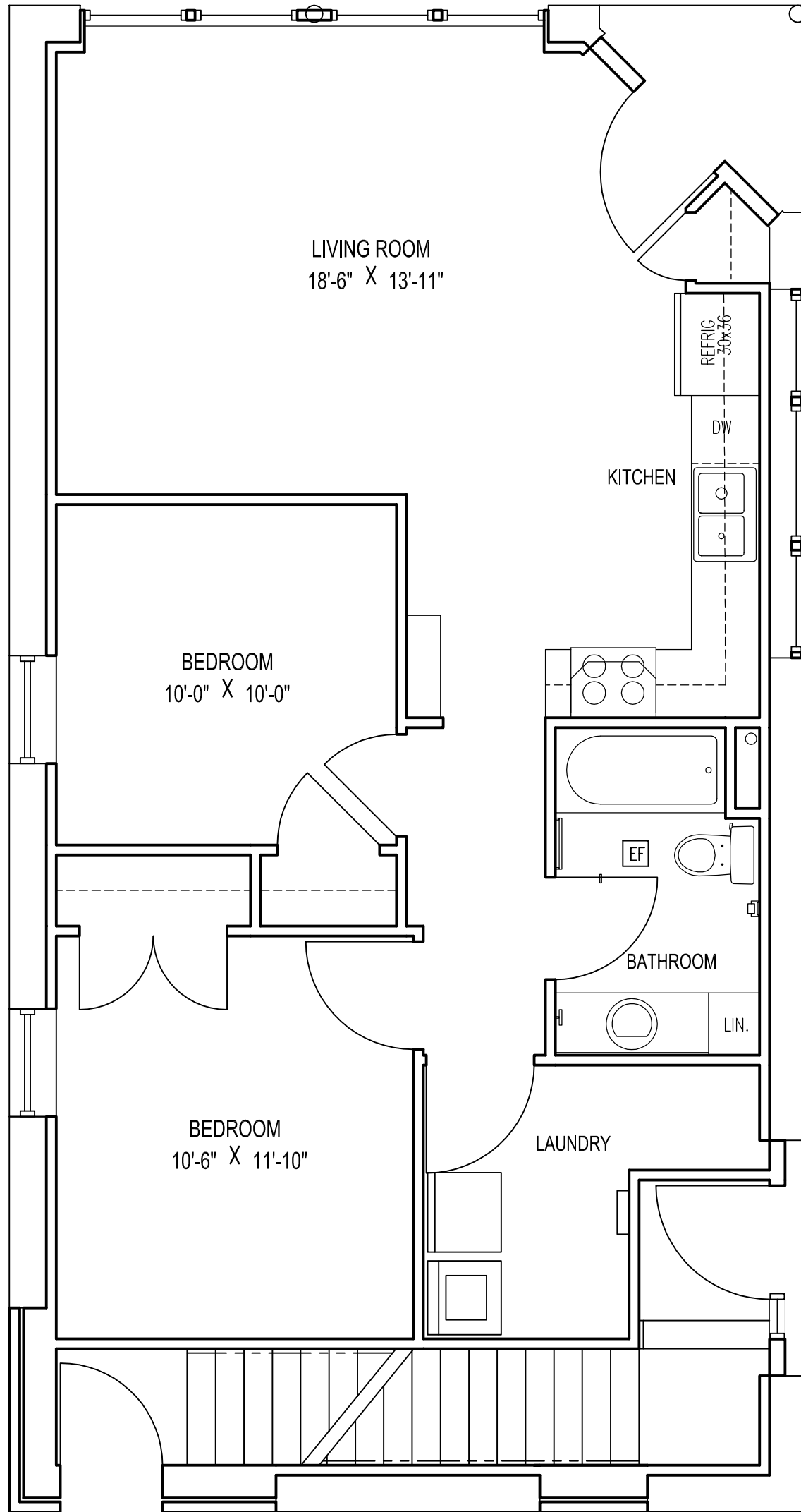
4100 ST. FERDINAND GARDEN UNIT - 1ST FLOOR
