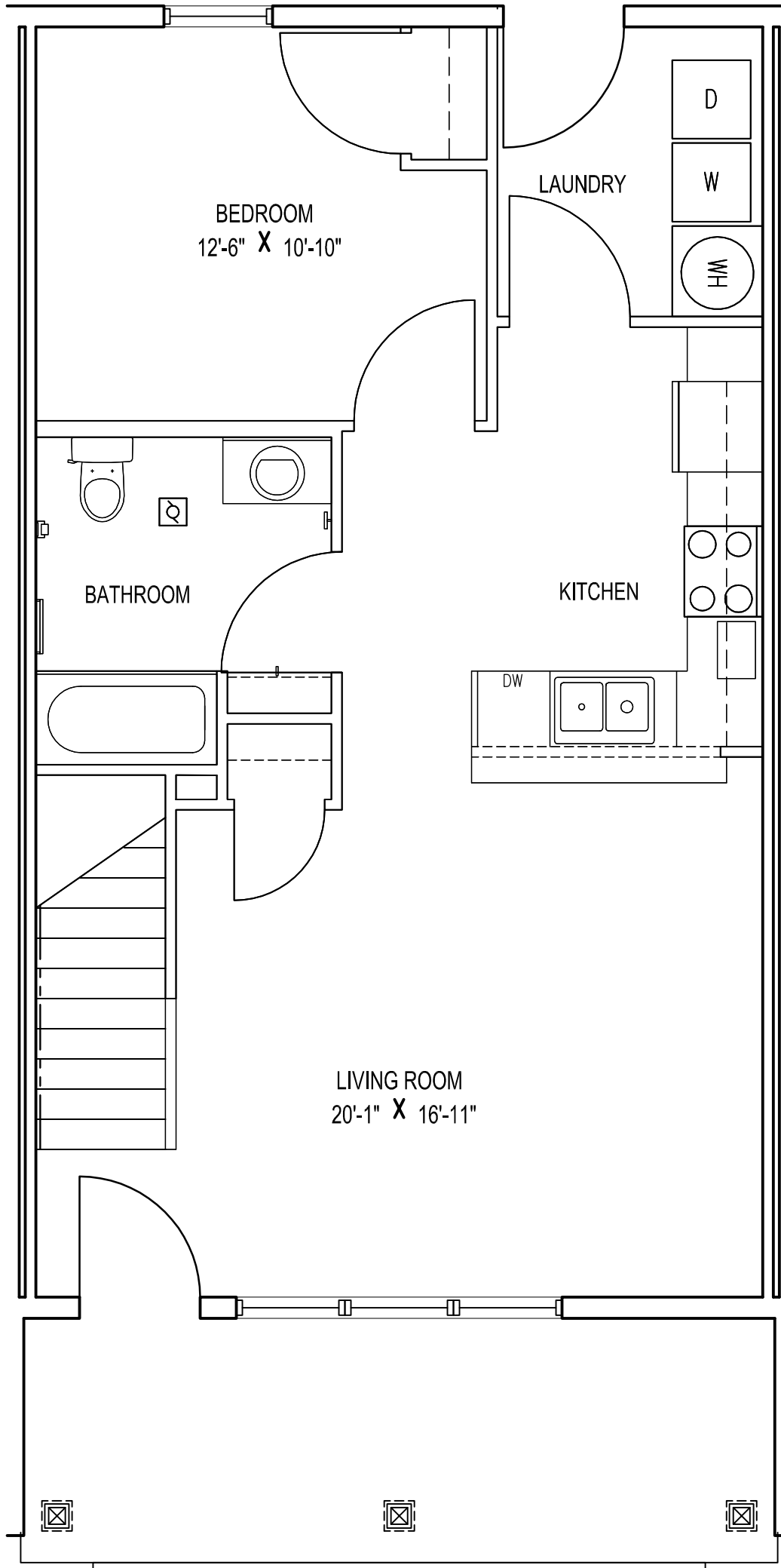
NEW CONSTRUCTION TOWNHOME 4 - 1ST FLOOR
