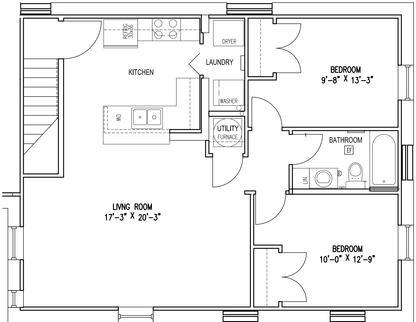
2510 N. SARAH GARDEN UNIT - 2ND FLOOR
